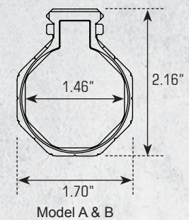
RB-HP25B (4/PACK) Low Profile Keymod Rail Panel Covers [Also Refer to P. 153]
