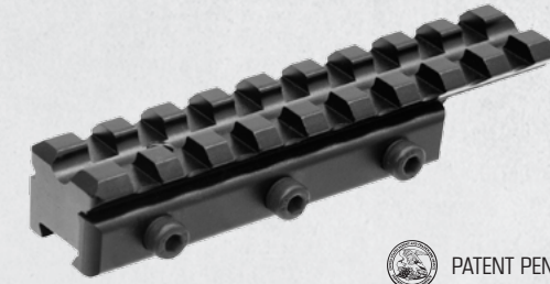
MNT-PMTOWL-A Dovetail to Picatinny Adaptor Mount • Precision Machined from Aircraft Aluminum with a Matte Black Finish • 3.94" Scalloped 9 Slot Picatinny Rail with 0.59" Saddle Height • Compatible with Flat Receivers Equipped with 9mm-11mm Dovetail Rails
