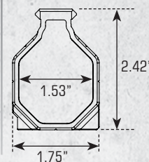
MR556 RAIL
